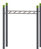
SWC.4251 Hangelleiter / Monkey bars M/D 210 x 150 x 270 cm H 120 cm
